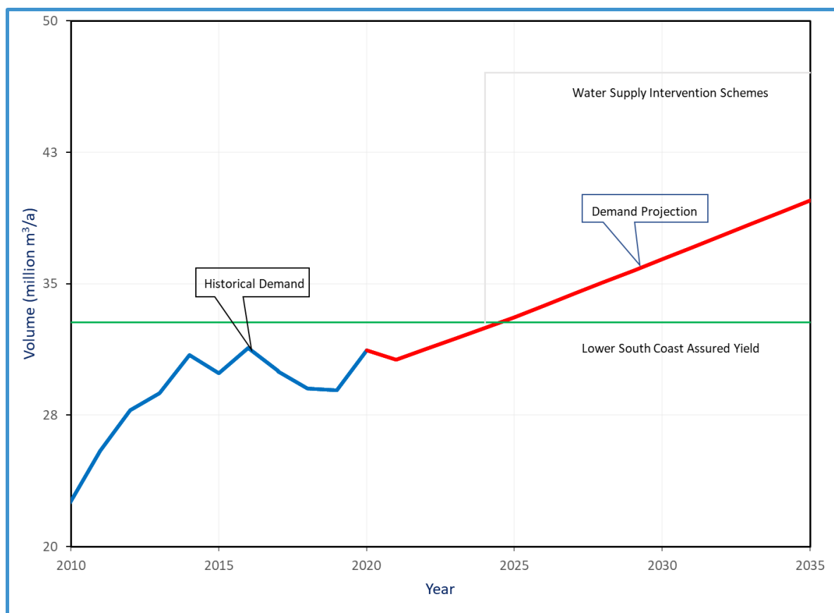
Figure 11.25 Lower South Coast water requirement projection scenarios.
