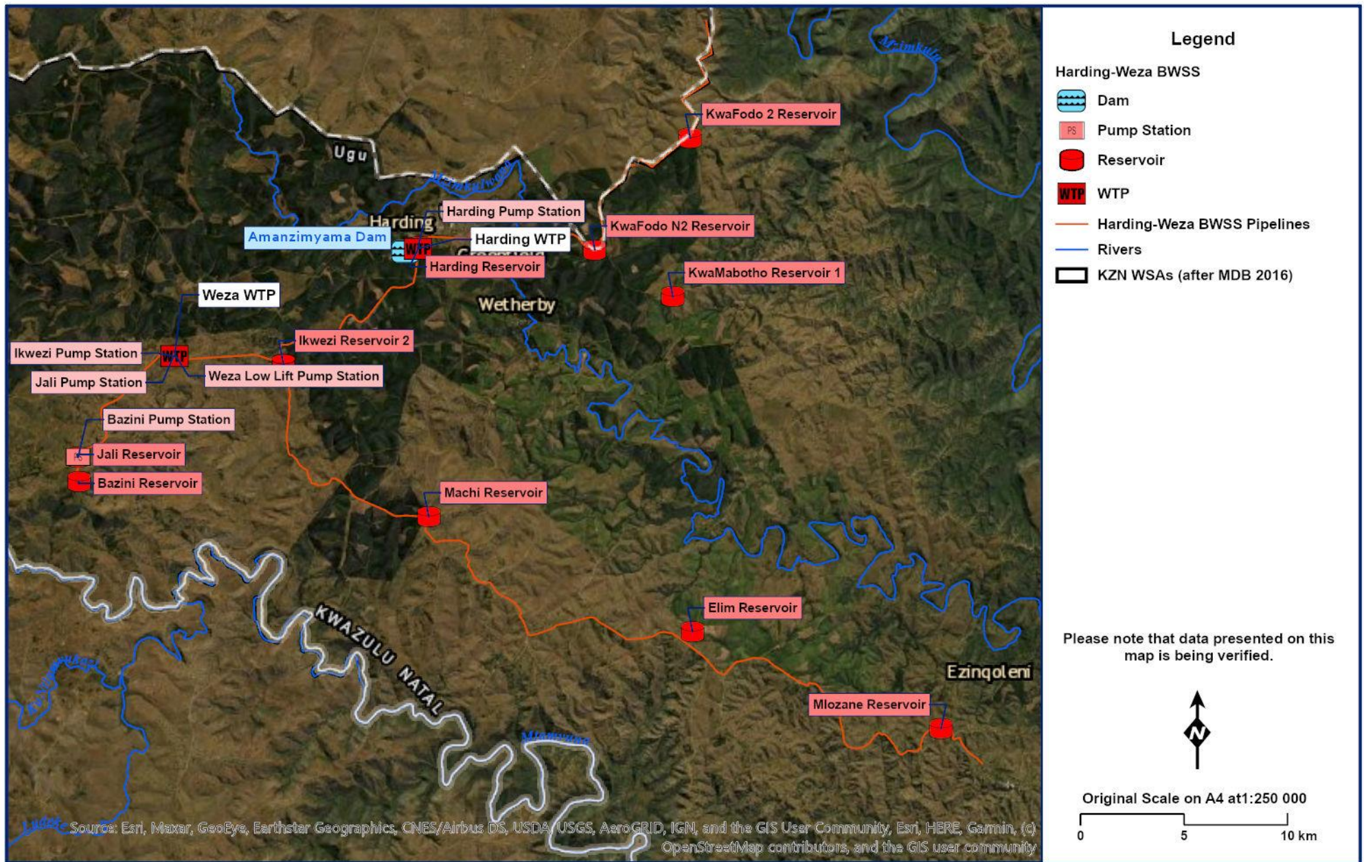
Figure 11.11 Harding-Weza Supply System.
