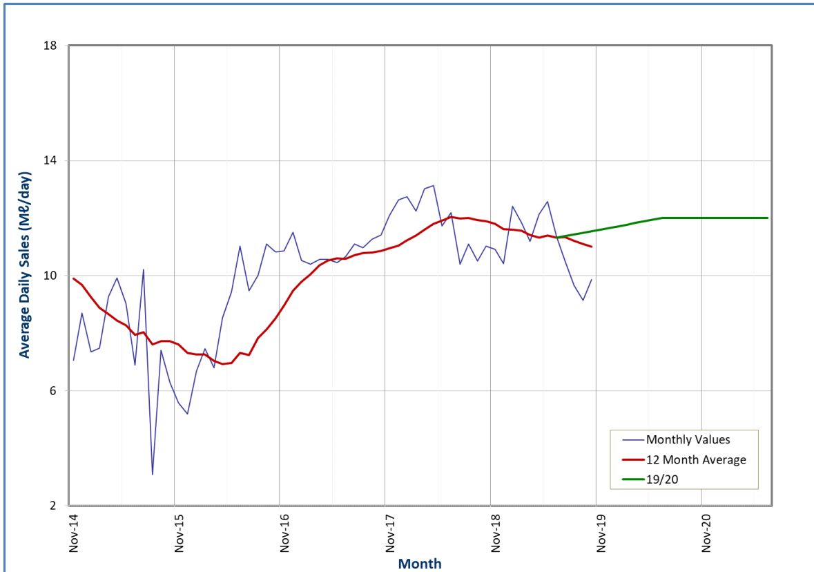
Figure 11.41 Water demand from Umzinto WTP.
