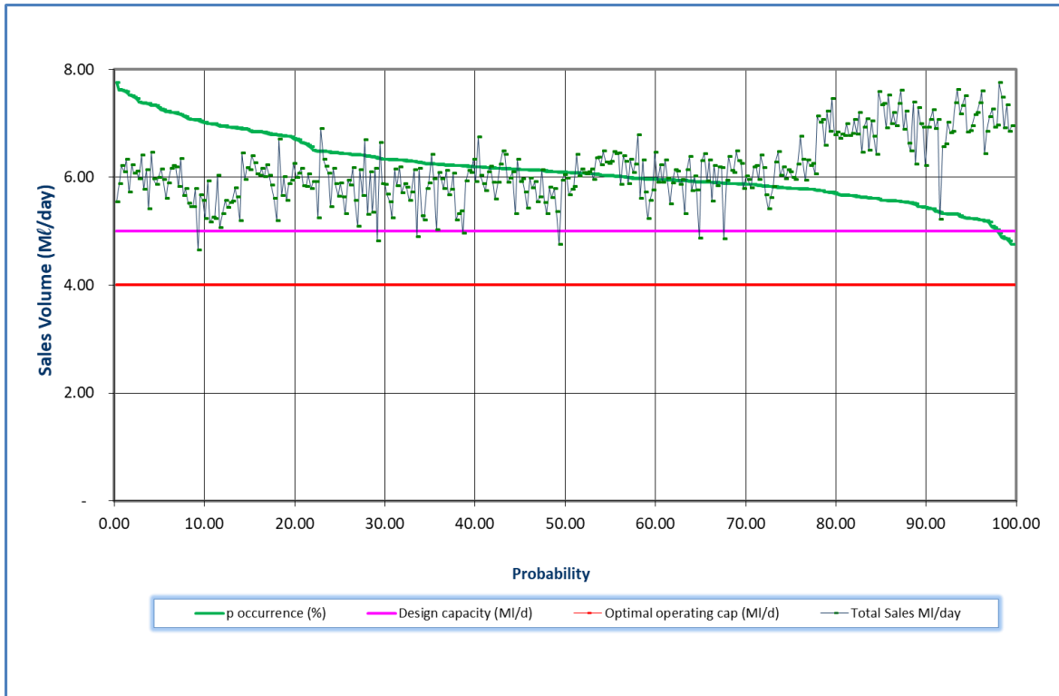
Figure 11.33 Analysis of historical production at Mhlabatshane WTP (November 2018 to October 2019).
