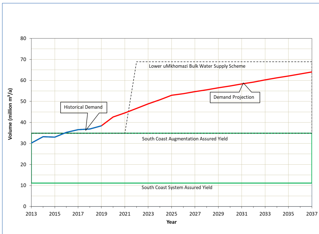
Figure 11.44 South Coast water requirement projection scenarios.
