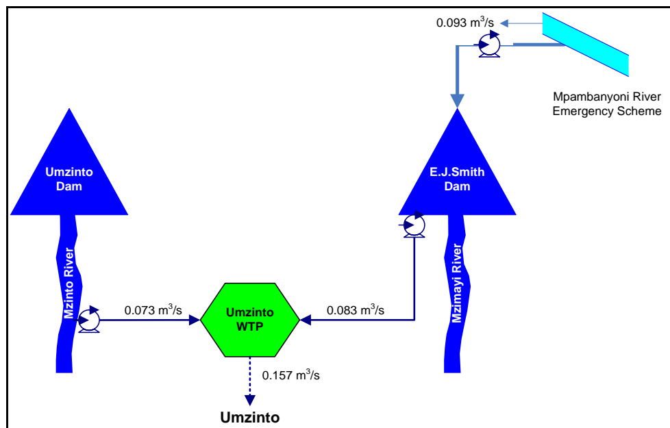
Figure 11.22 Schematic of the Middle South Coast system.
