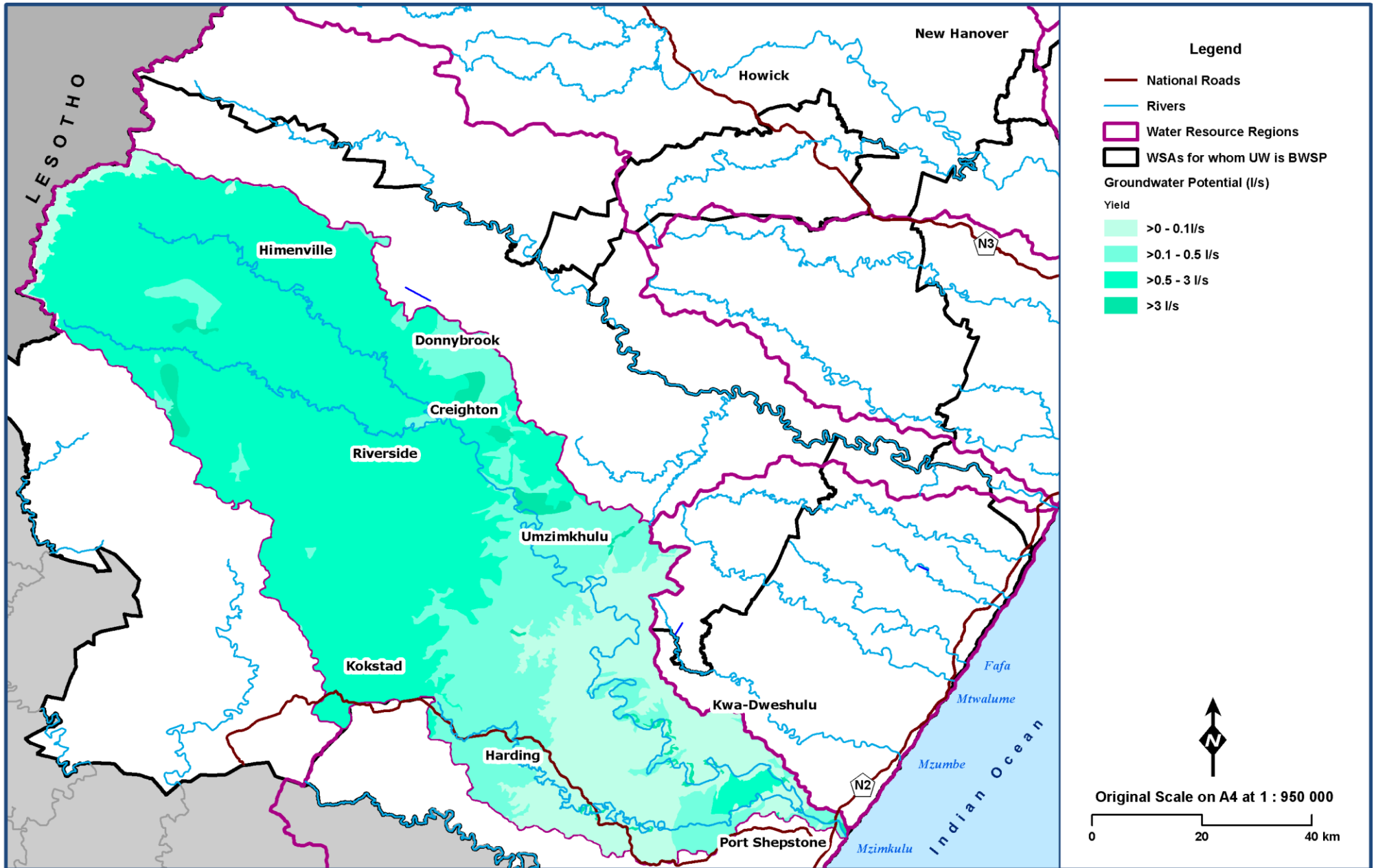
Figure 11.13 Groundwater potential in the Mzimkulu Region (KZN DoT 2011; MDB 2016; Umgeni Water 2017; WR2012).
