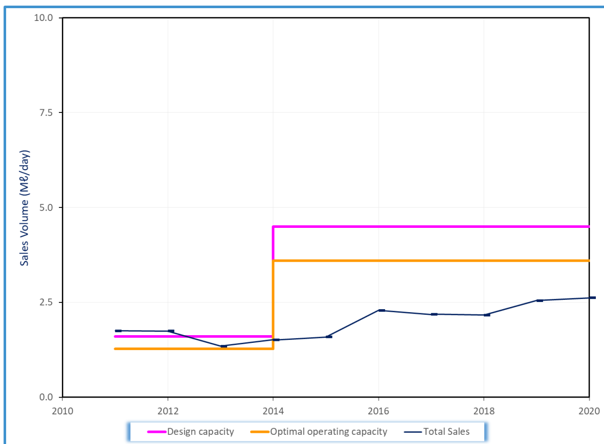
Figure 11.16 Analysis of historical production at Vulamehlo WTP (January 2010 to January 2020).
