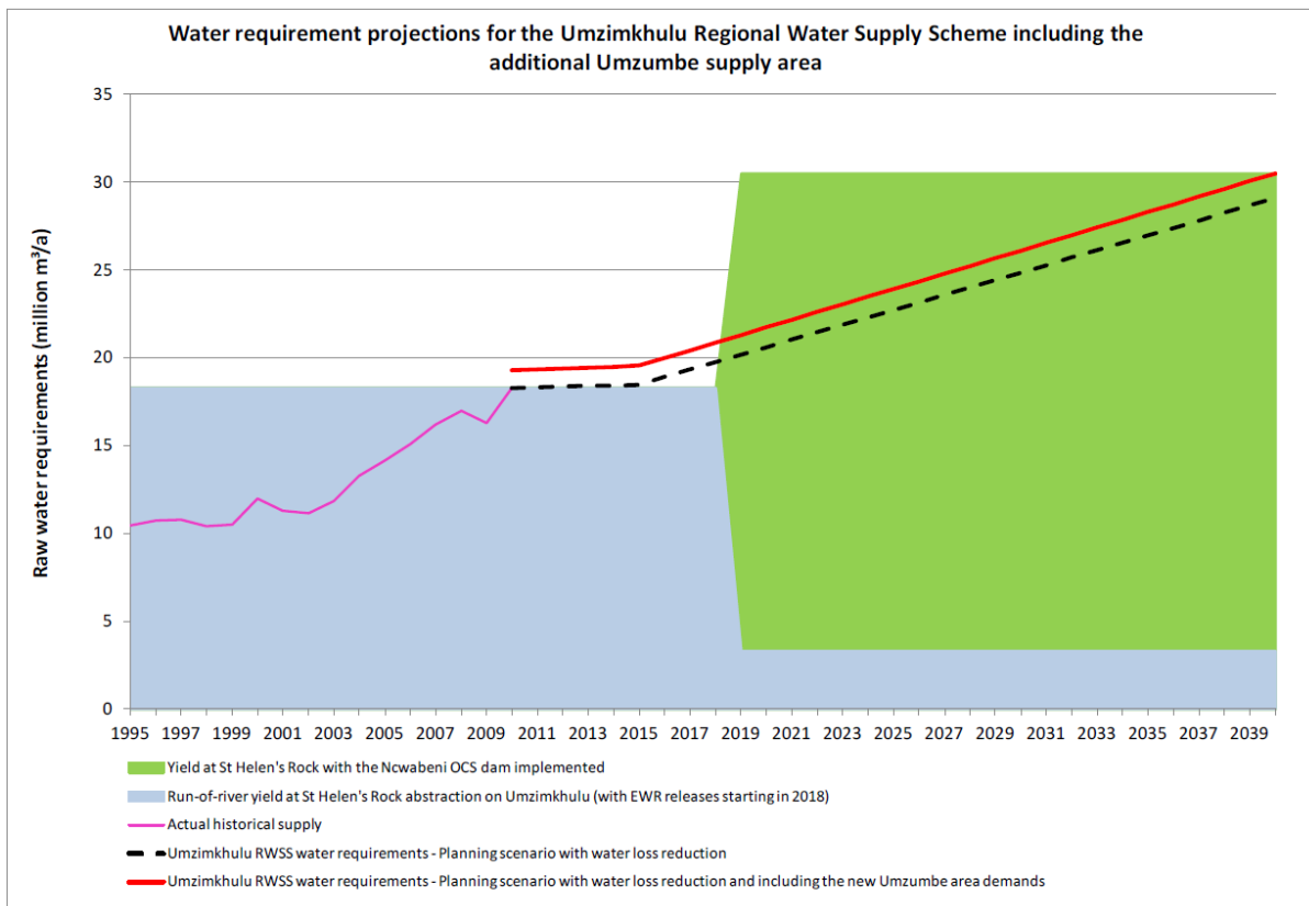
Figure 11.27 Water Balance Lower South Coast.
