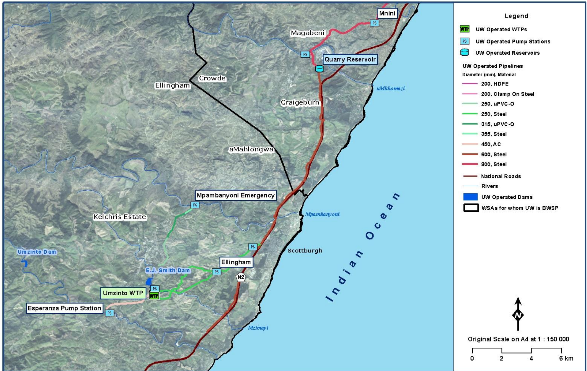
Figure 11.27 Umzinto Supply System.
