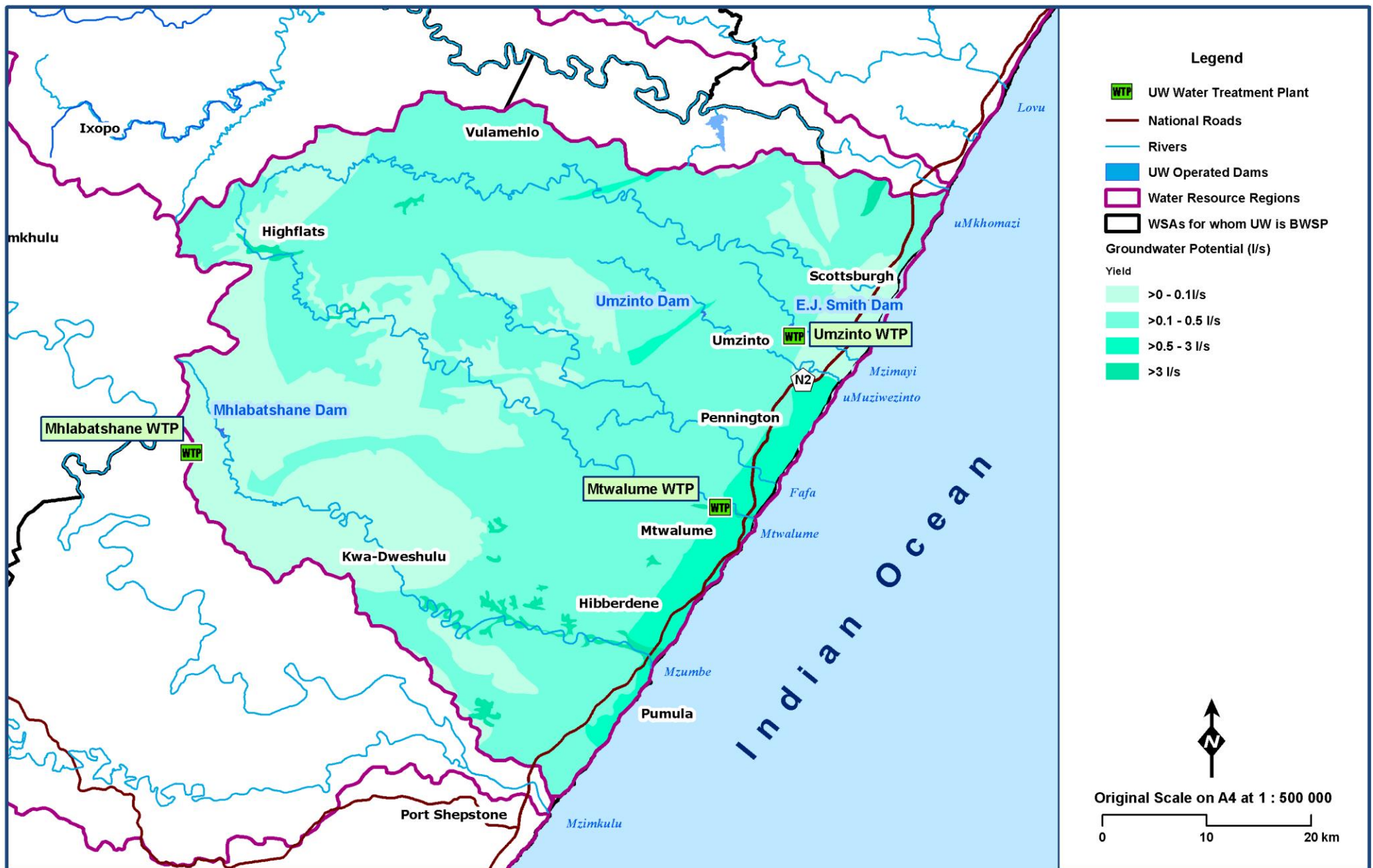
Figure 11.8 Groundwater potential in the Middle South Region (KZN DoT 2011; MDB 2016; Umgeni Water 2017; WR2012).
