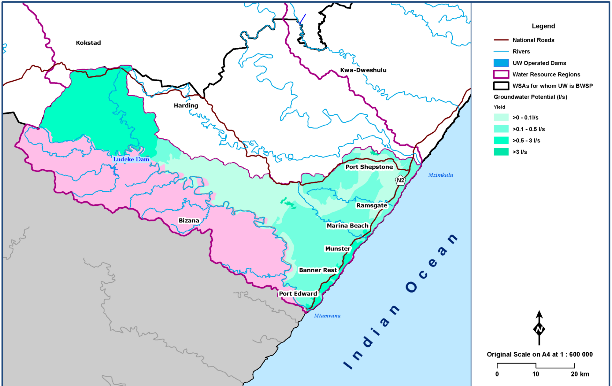
Figure 11.15 Groundwater potential in the Mtamvuna Region (KZN DoT 2011; MDB 2016; Umgeni Water 2017; WR2012).
