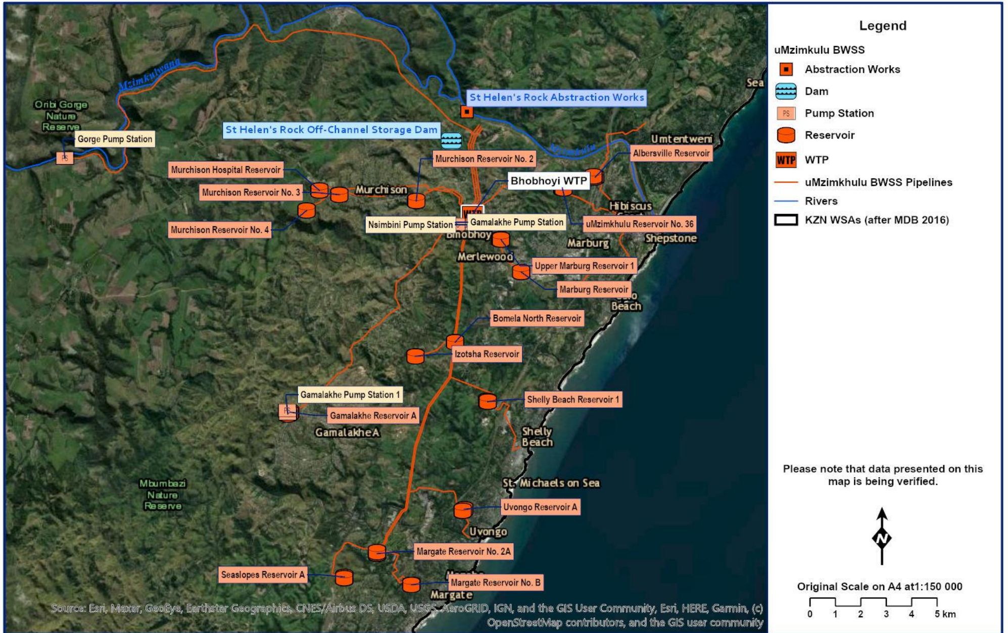
Figure 11.9 uMzimkhulu Supply System.
