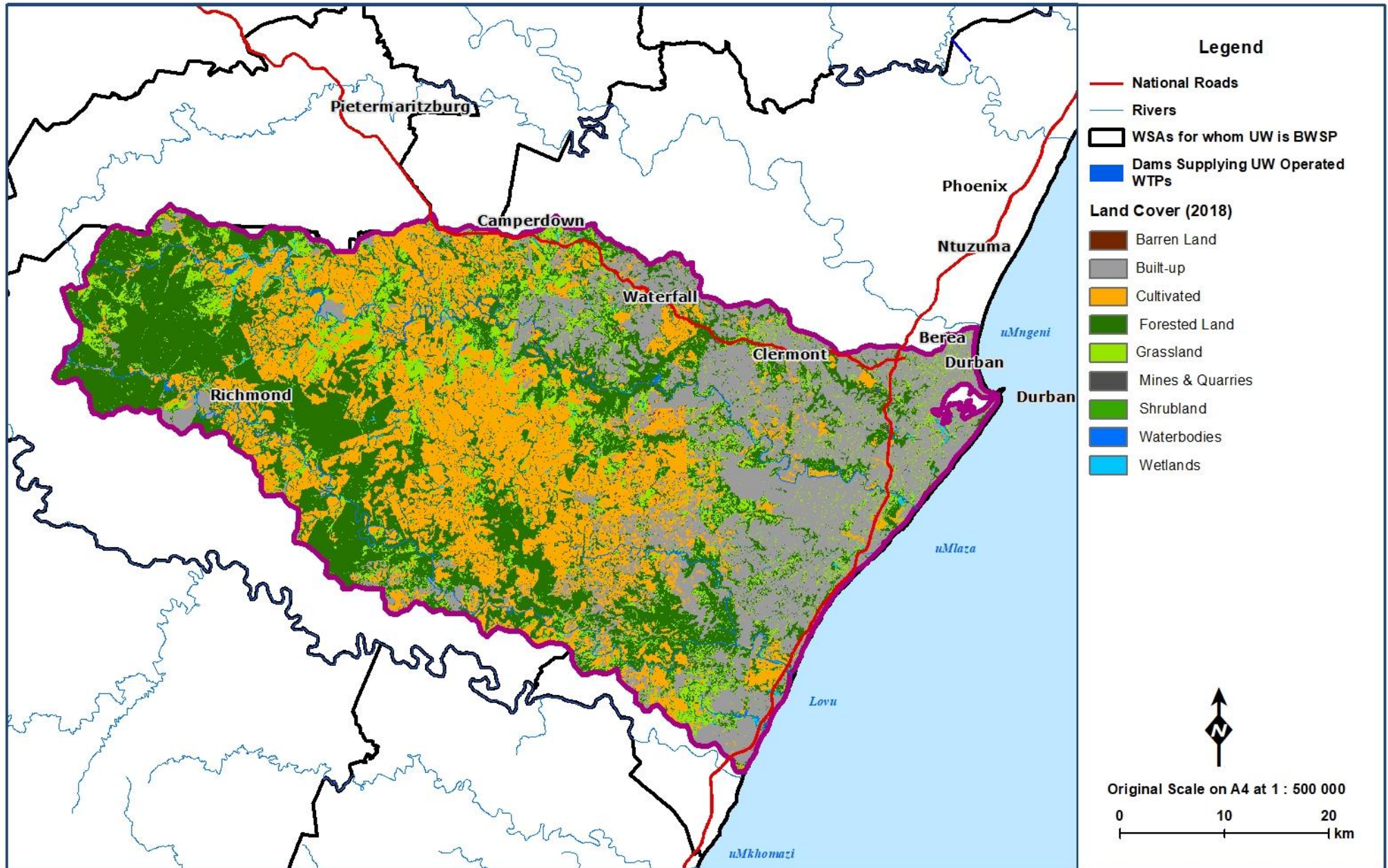
Figure 11.4 General layout of the Mlazi/Lovu Region (DEA and GTI 2018; KZN DoT 2017; MDB 2016; Umgeni Water 2020; WR2012).
