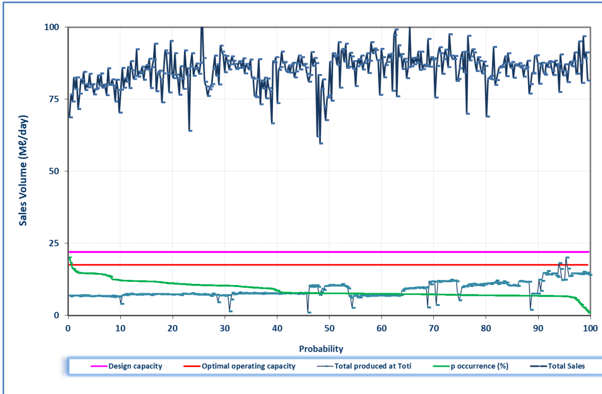
Figure 11.30 Analysis of historical production at Amanzimtoti WTP (November 2018 to October 2019).
