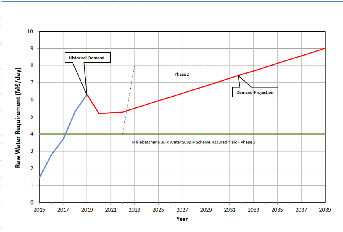
Figure 11.48 Water Balance Mhlabatshane BWSS.
