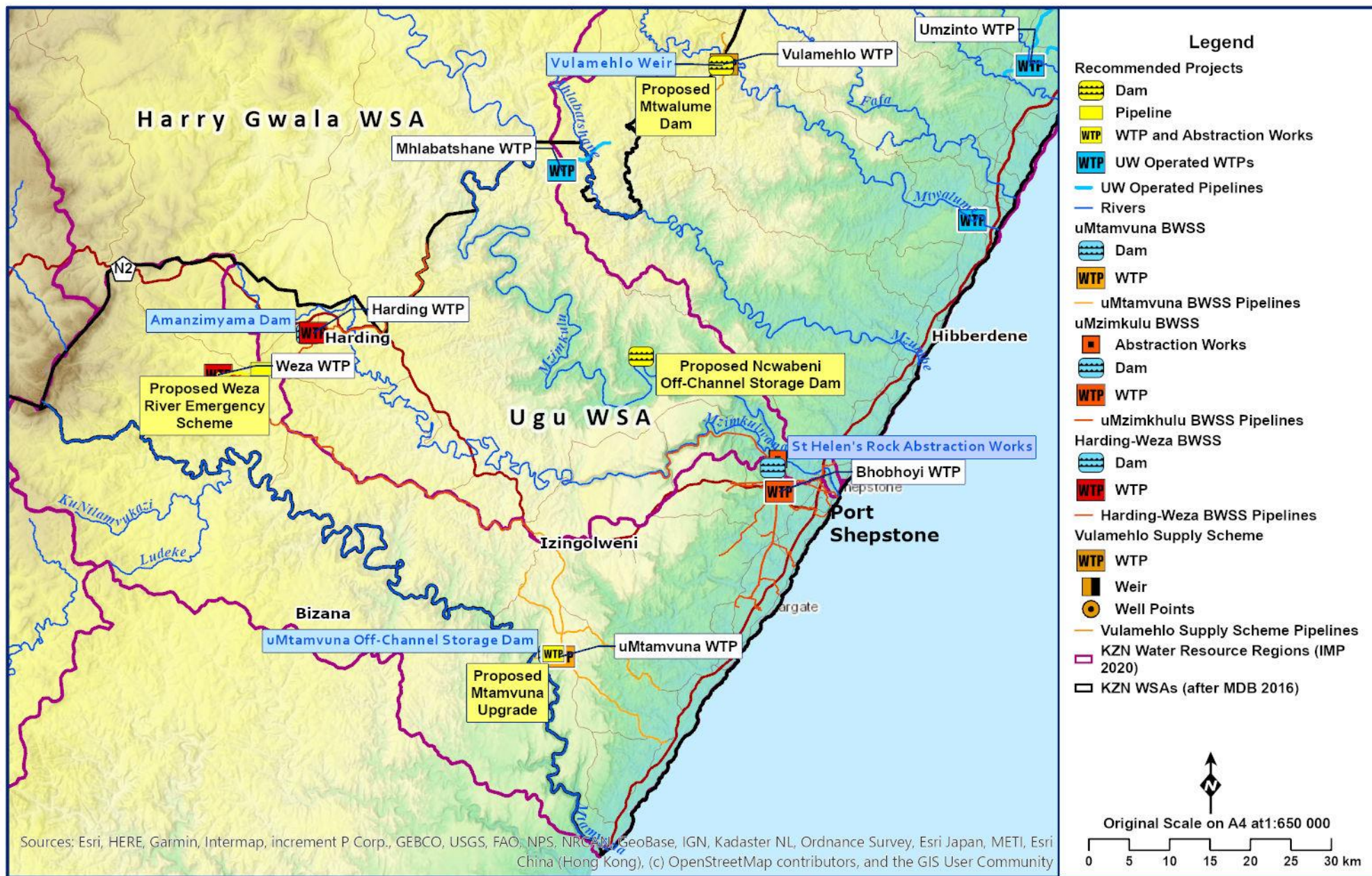
Figure 11.26 Proposed water resource infrastructure in the Lower South Coast Region (KZN DoT 2017; MDB 2016; Umgeni Water 2020; WR2012).
