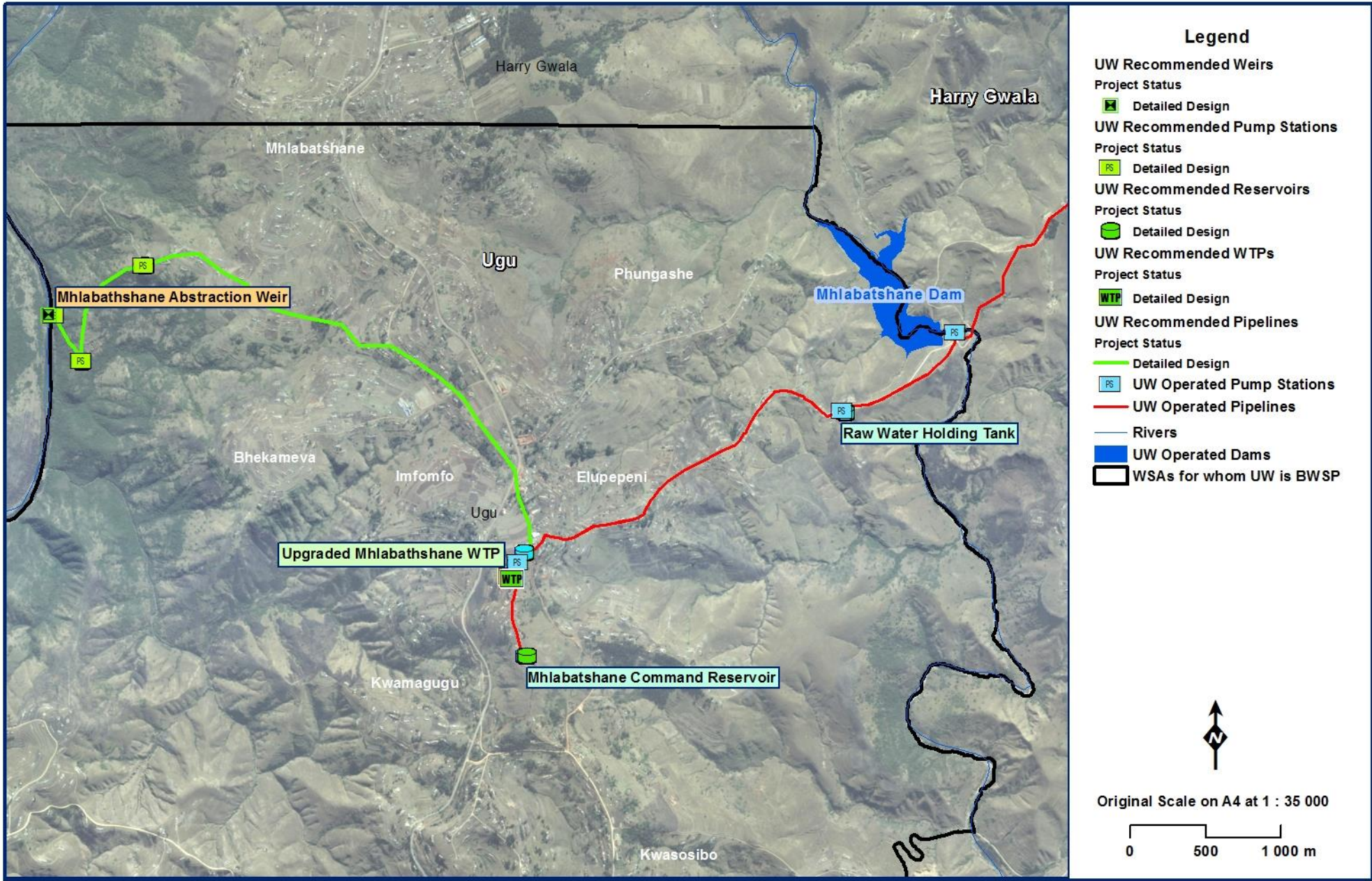
Figure 11.47 General layout of the Mhlabatshane BWSS Phase 2.
