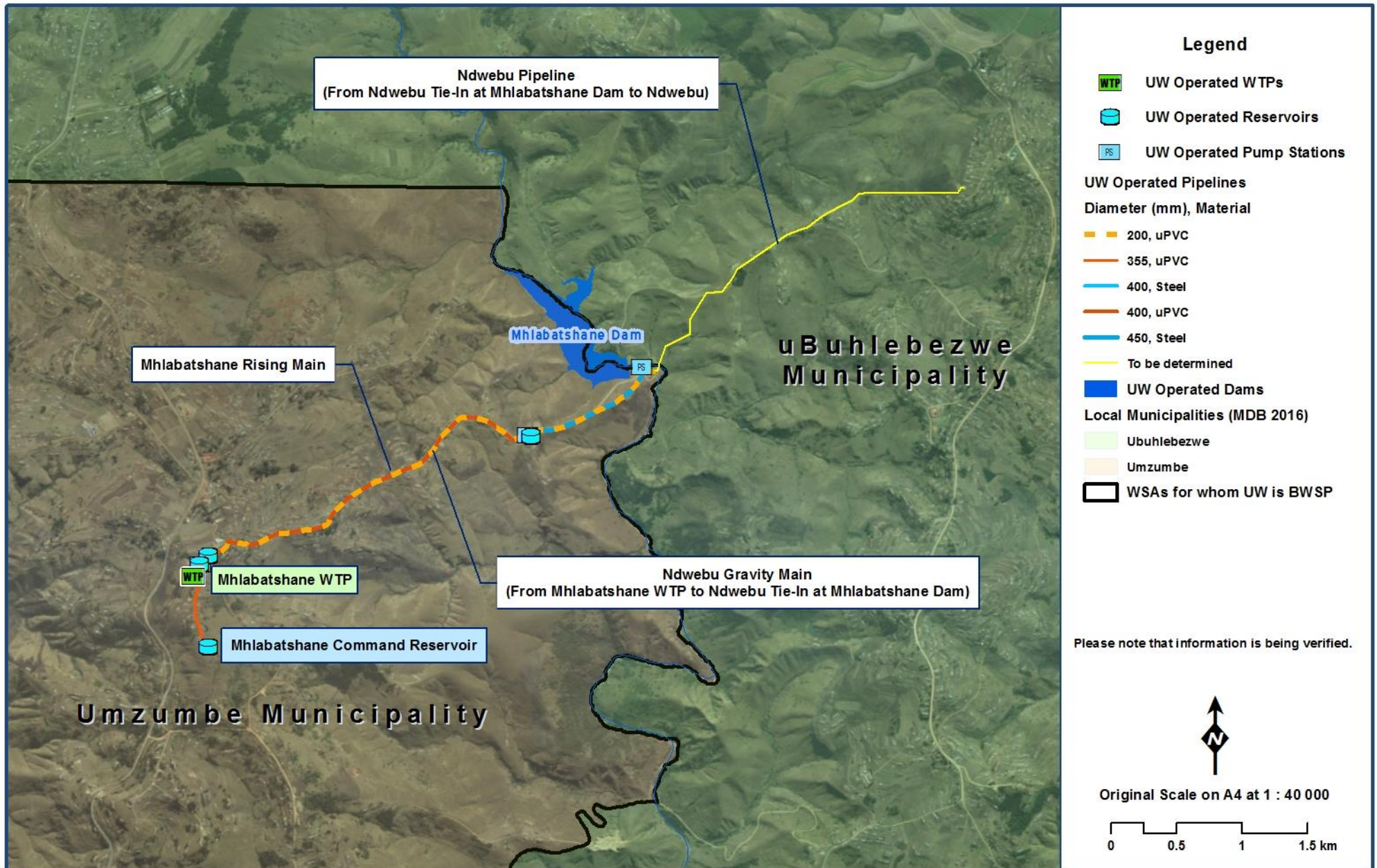
Figure 11.29 Mhlabatshane Supply System.
