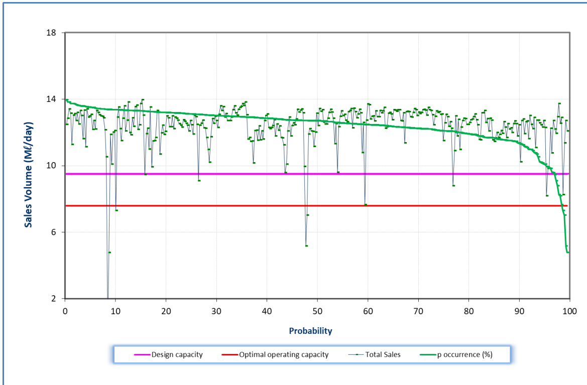
Figure 11.32 Analysis of historical production at Mtwalume WTP (November 2018 to October 2019).
