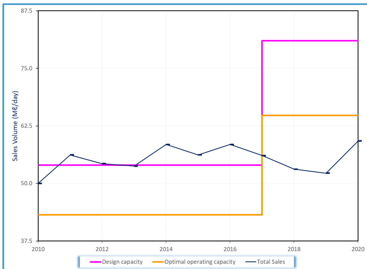
Figure 11.13 Analysis of historical production at Bhobhoi WTP (January 2010 to January 2020).
