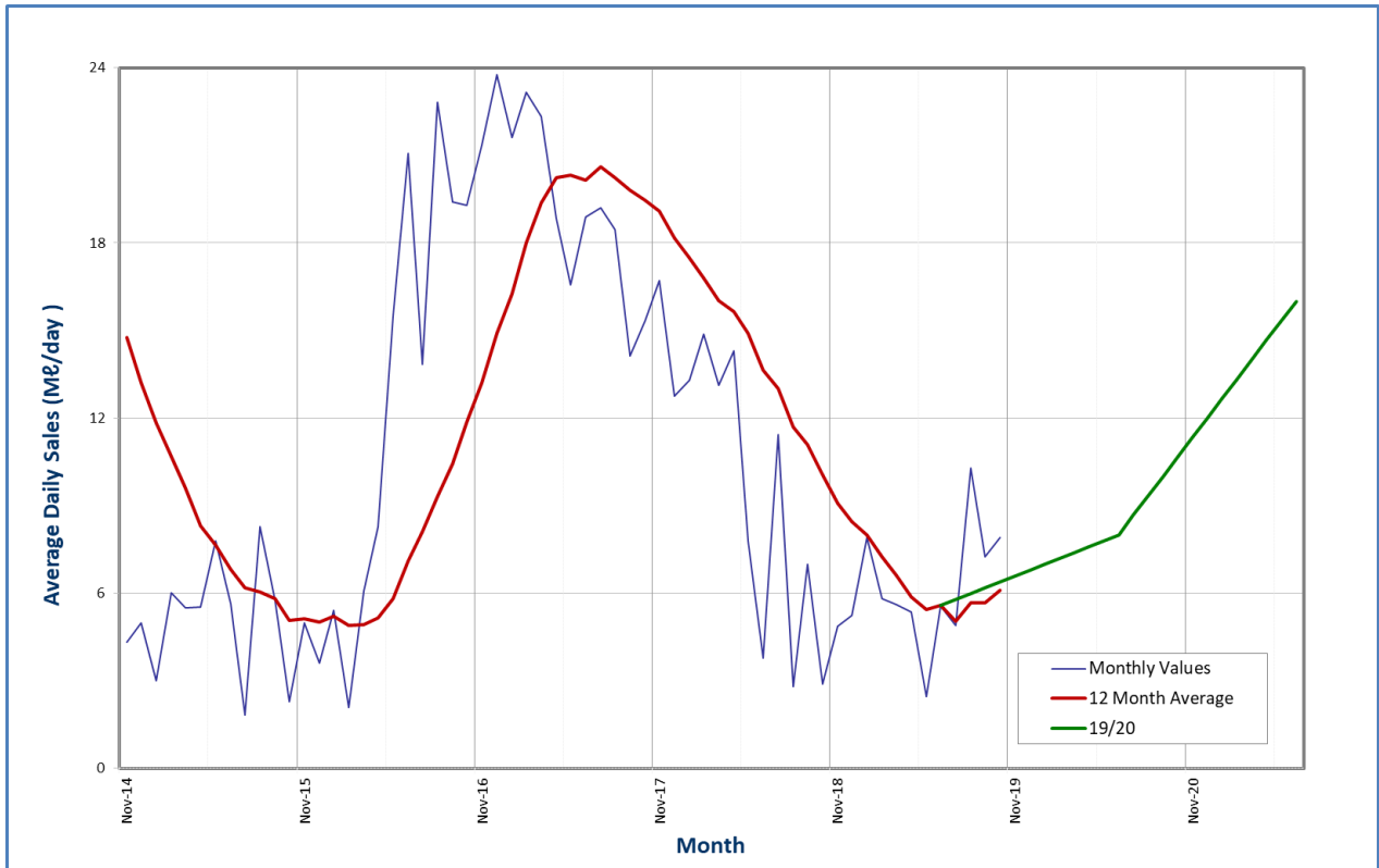
Figure 11.40 Water demand from Amanzimtoti WTP.
