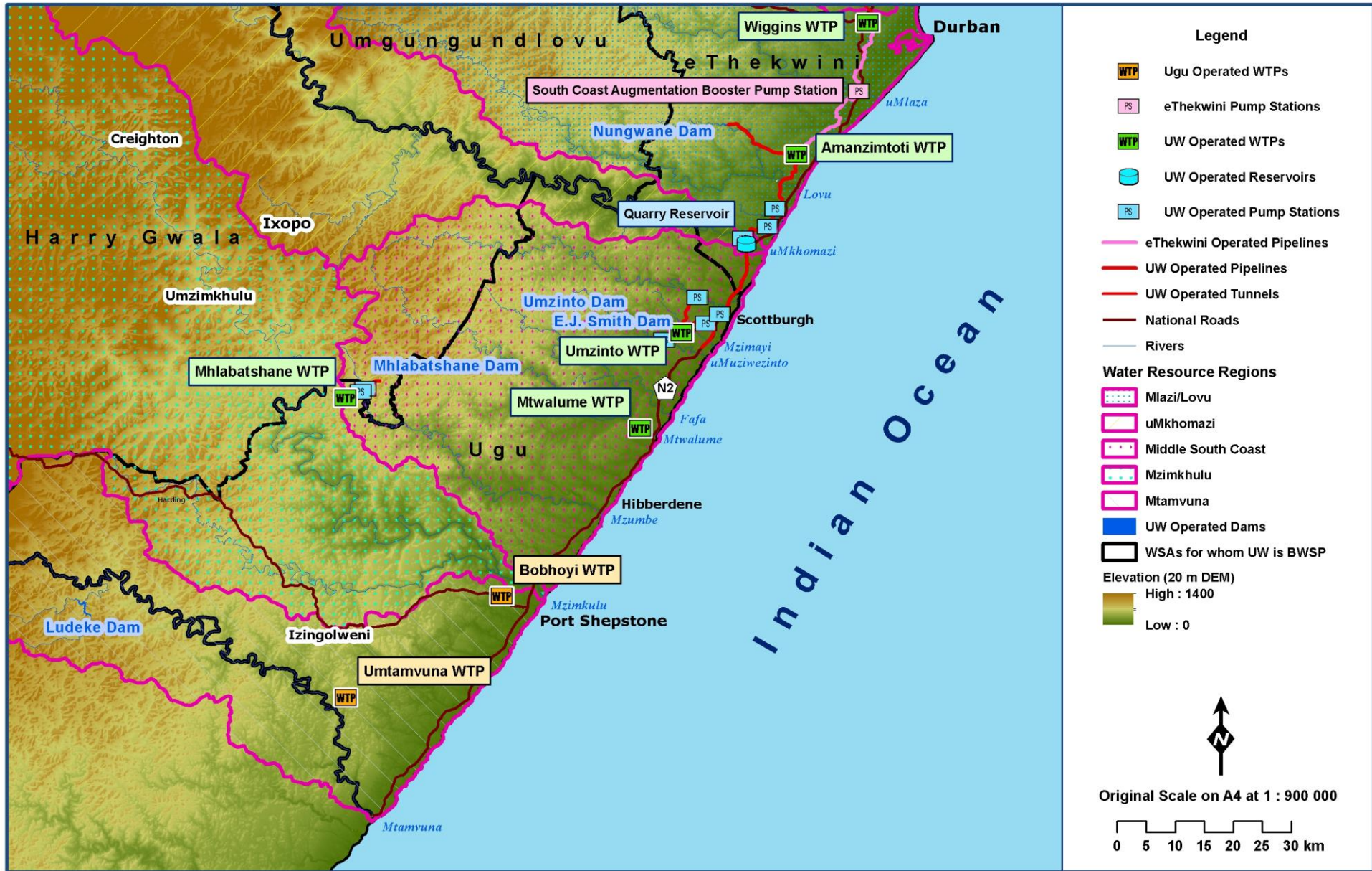
Figure 11.1 General layout of the South Coast System.
