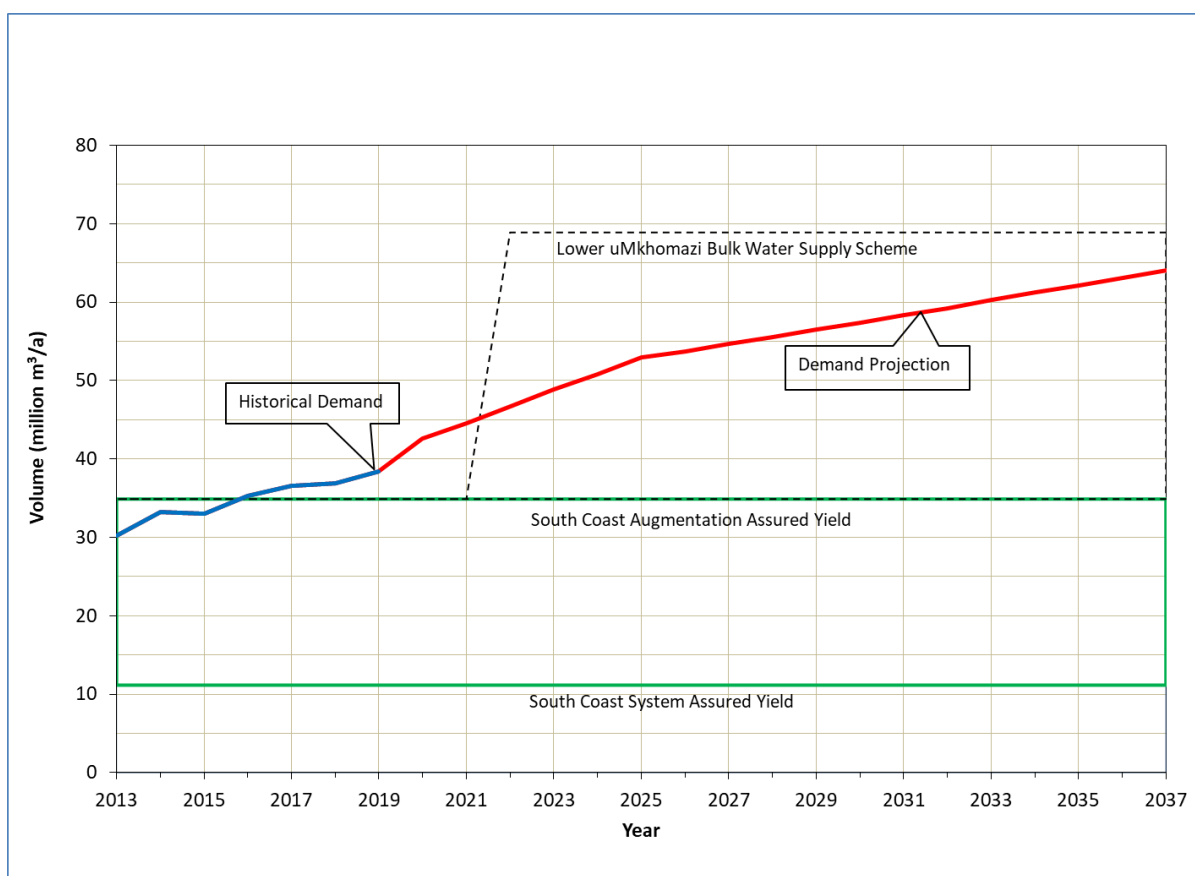
Figure 11.49 Water Balance Upper and Middle South Coast.
