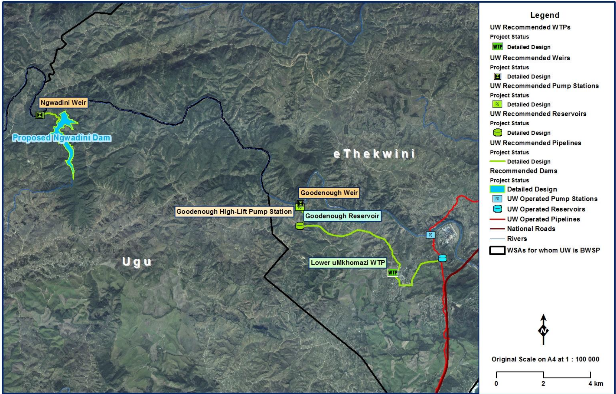
Figure 11.50 Layout of the proposed Lower uMkhomazi BWSS.
