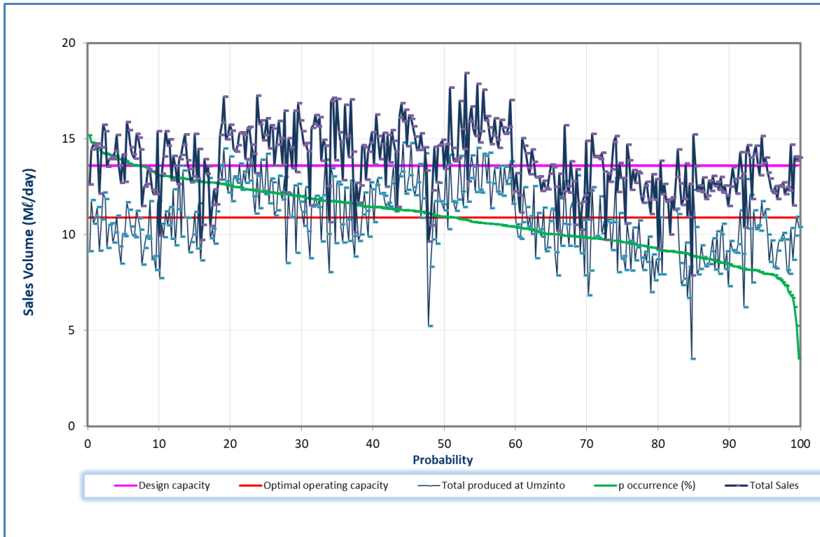
Figure 11.31 Analysis of historical production at Umzinto WTP (November 2018 to October 2019).
