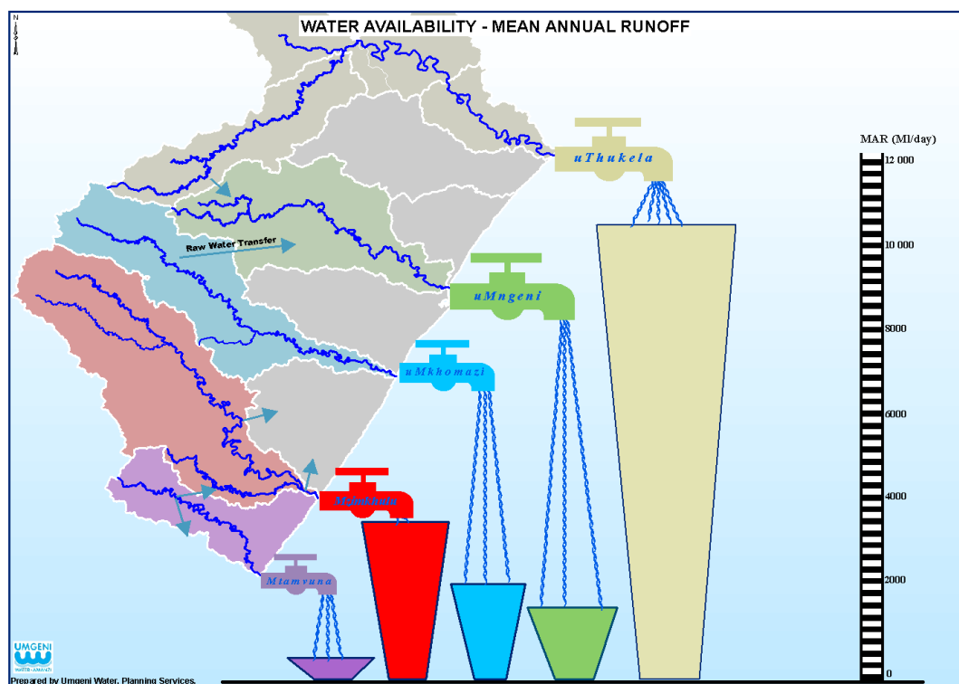
Figure 11.4 Water Availability – Mean Annual Runoff.
