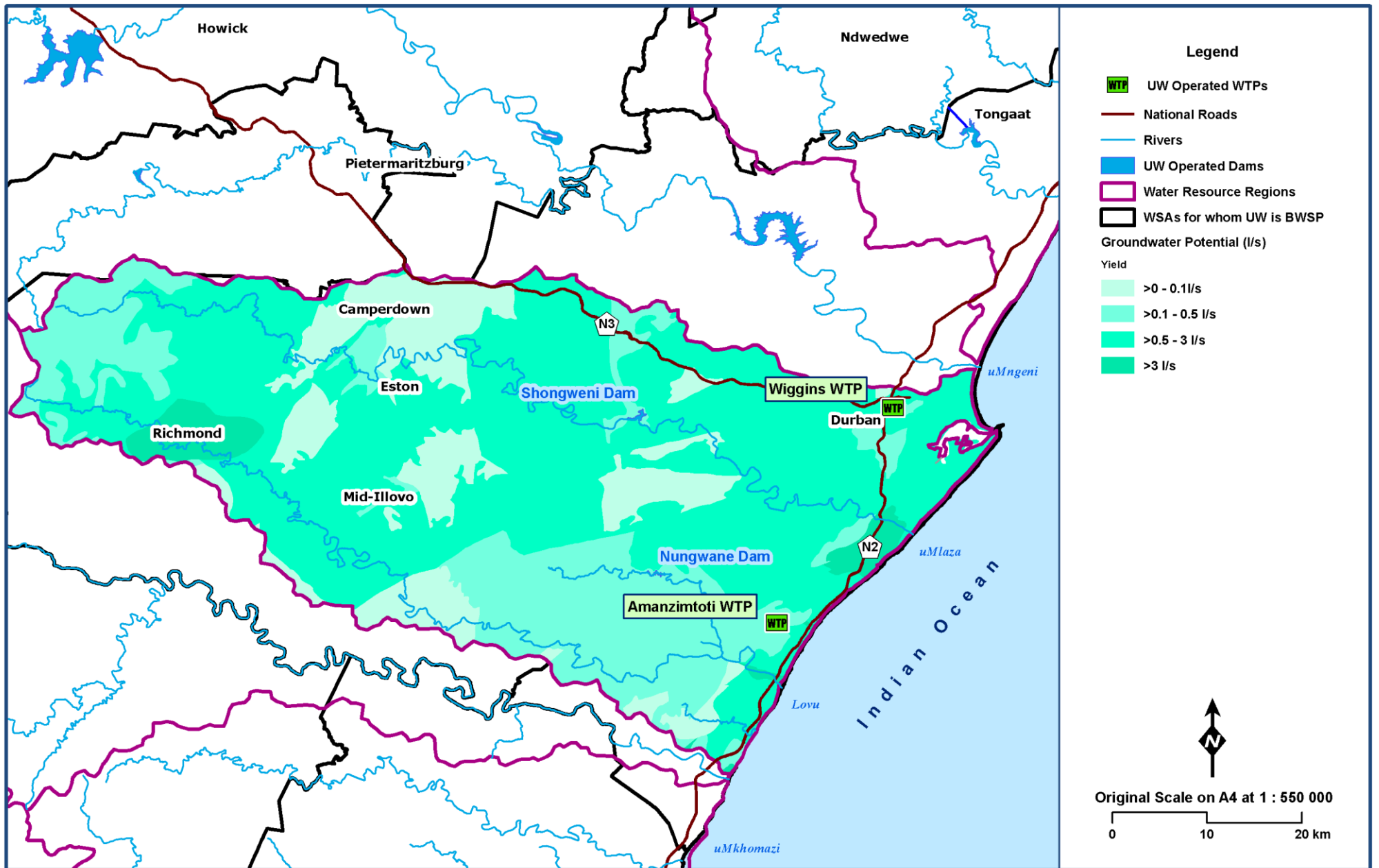
Figure 11.5 Groundwater potential in the Mlazi/Lovu Region (KZN DoT 2011; MDB 2016; Umgeni Water 2017; WR2012).
