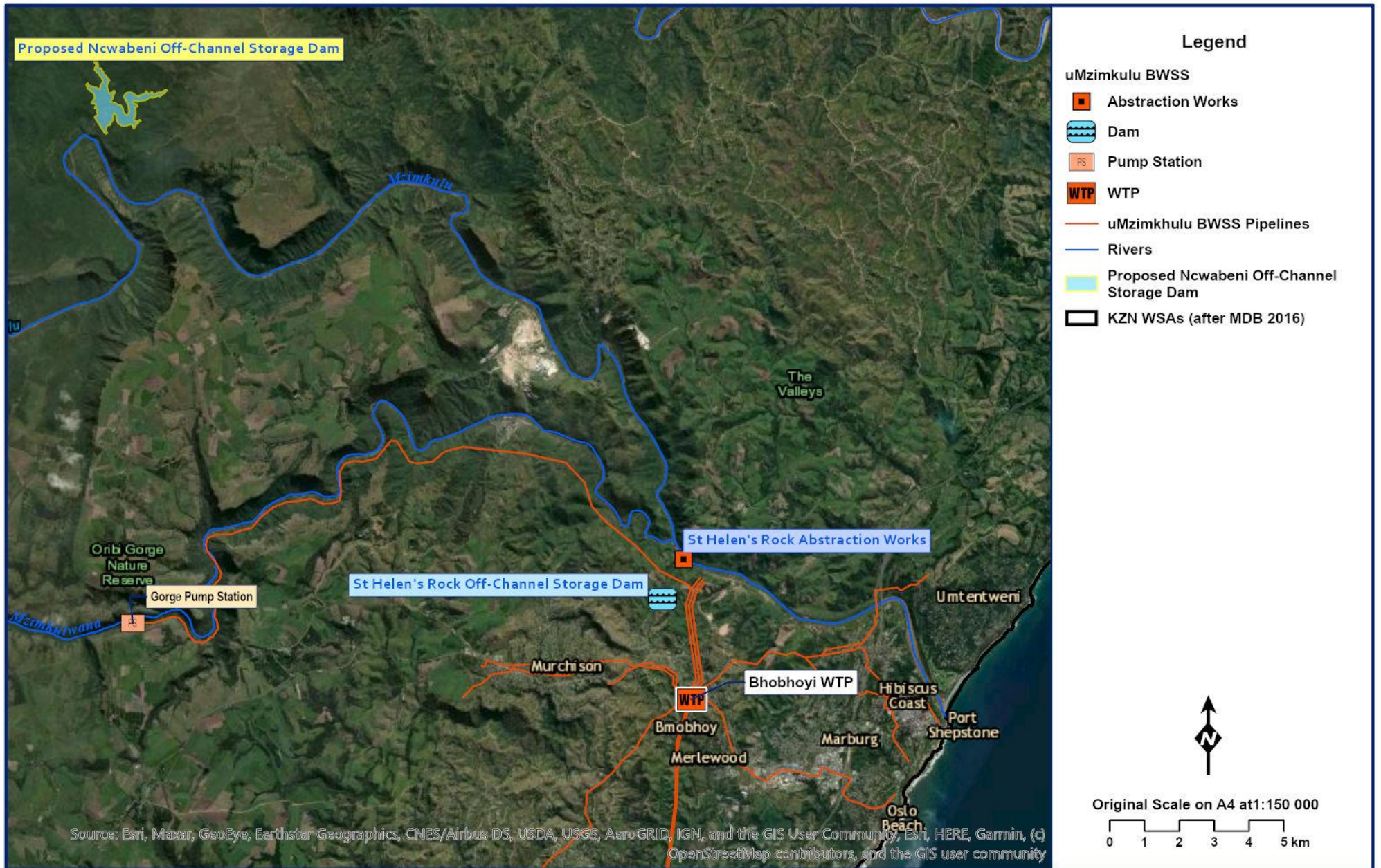
Figure 11.28 General layout of the Ncwabeni OCS Dam and Abstraction Work.
