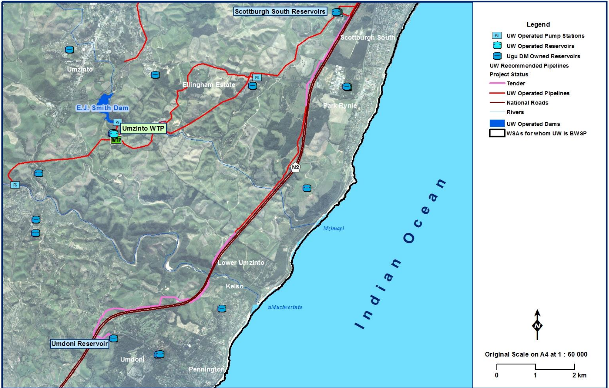
Figure 11.46 General layout of the proposed South Coast Pipeline Phase 2b.
