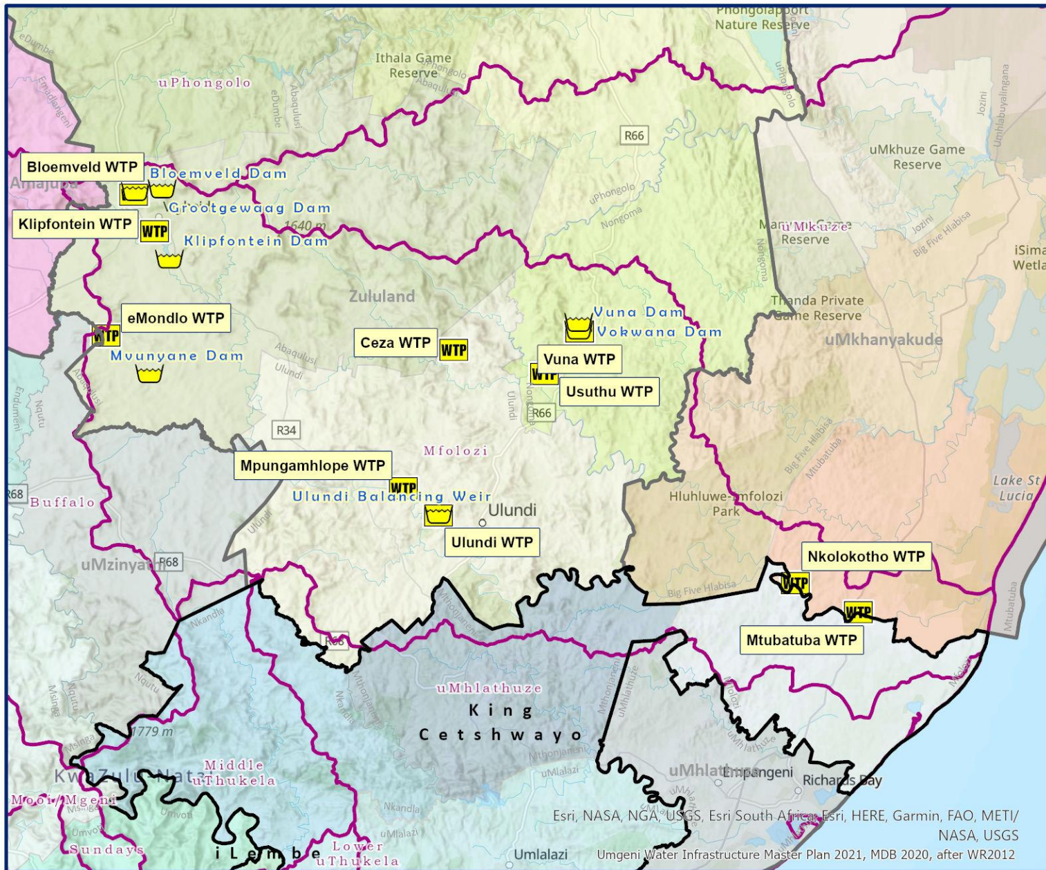
Figure 17.1 General layout of the Mfolozi System (MDB 2020, UW IMP 2021).
