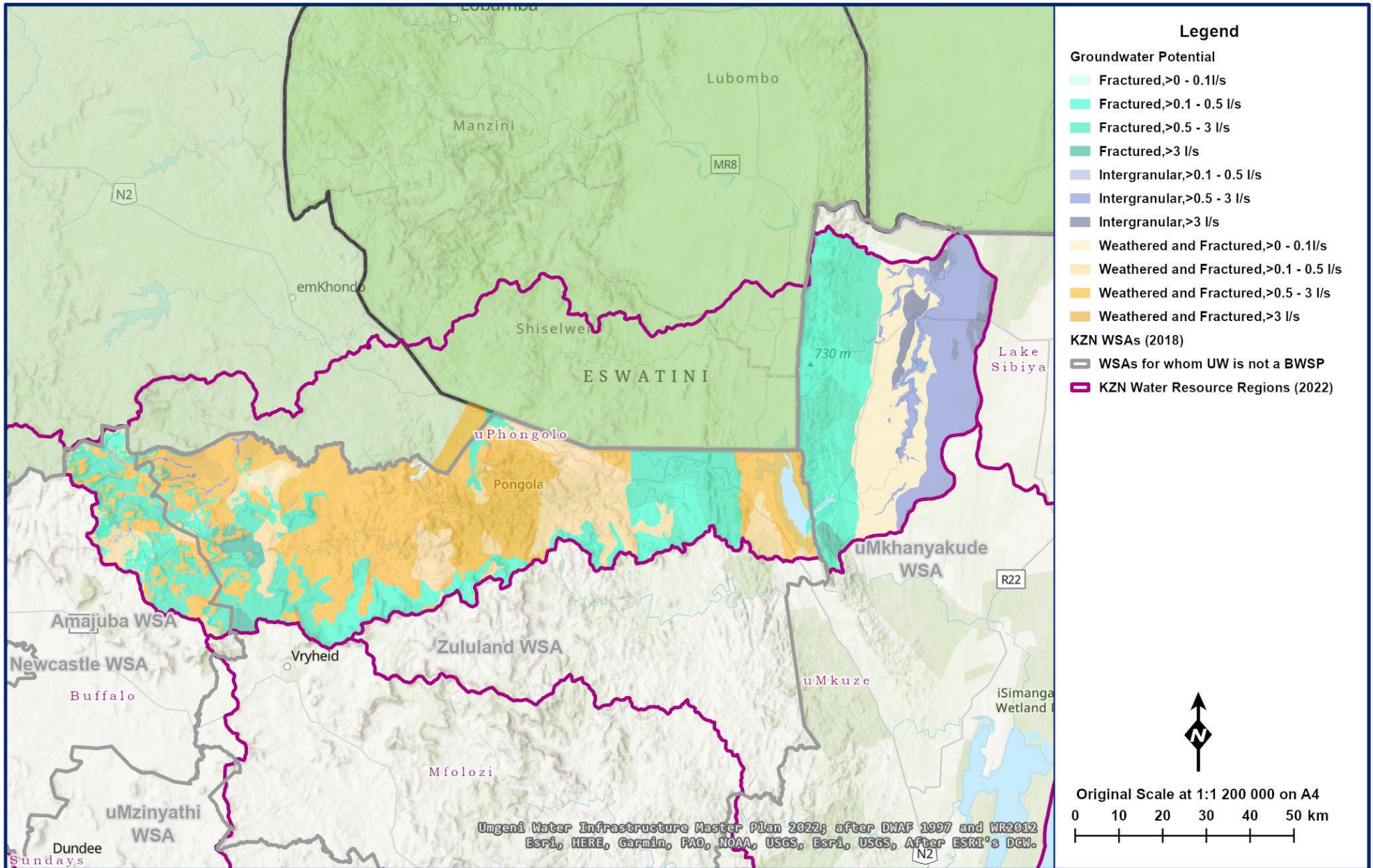
Figure 17.37 Groundwater potential in the Phongola Water Resource Region (MDB 2020, Umgeni Water 2022, after DWA 1997 and WR2012).
