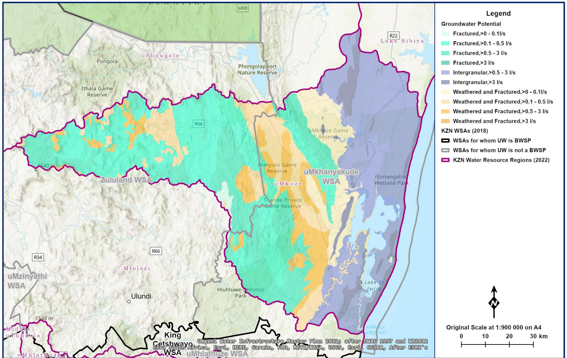
Figure 17.36 Groundwater potential in the uMkhuzo Region (MDB 2020, Umgeni Water 2021, after DWAF 1997 and WR2012).
