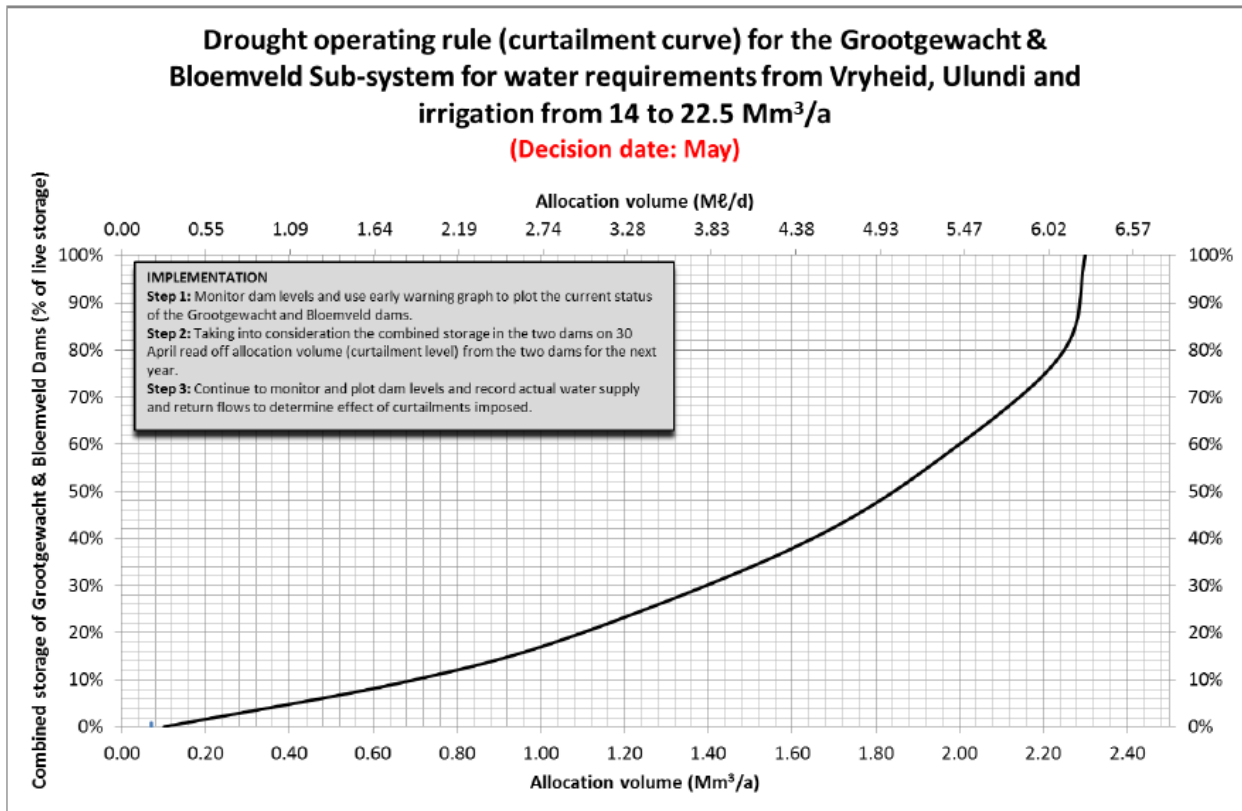
Figure 17.11 Drought operating rule for Grootgewacht & Bloemveld sub-system for Vryheid – May decision month (DWS, 2013)
