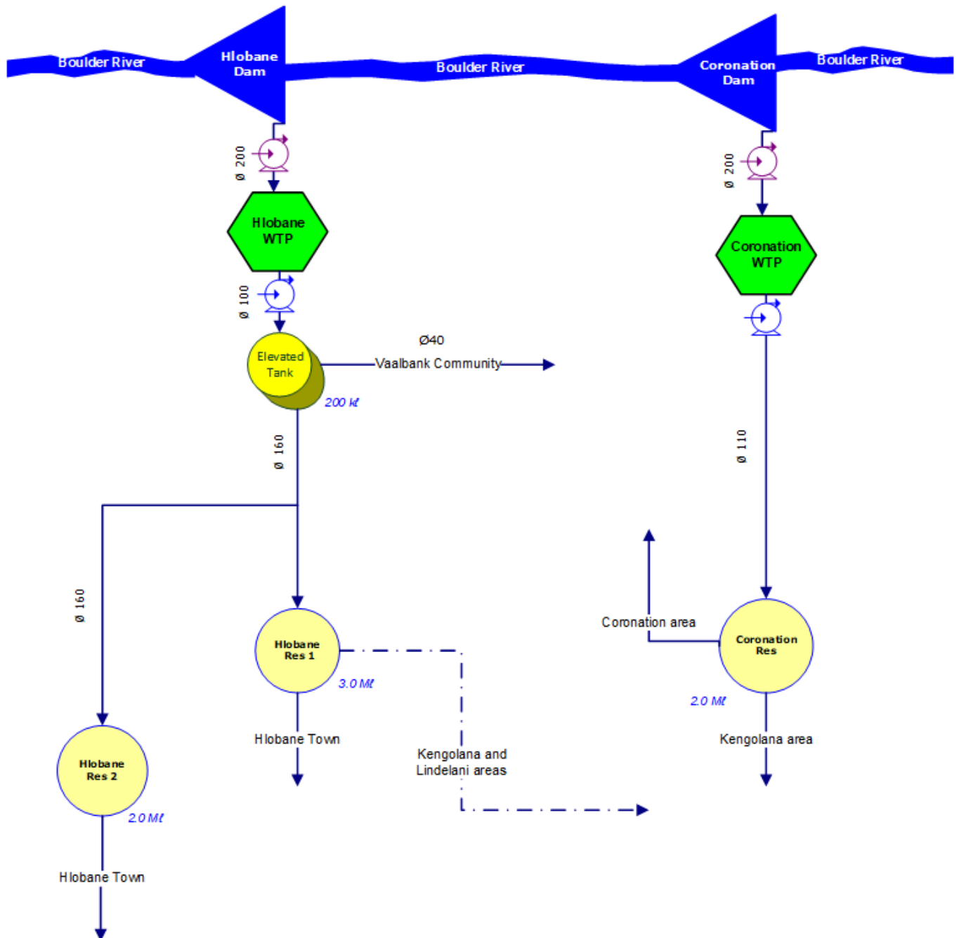
Figure 17.49 Schematic of the Hlobane/Coronation Supply System.
