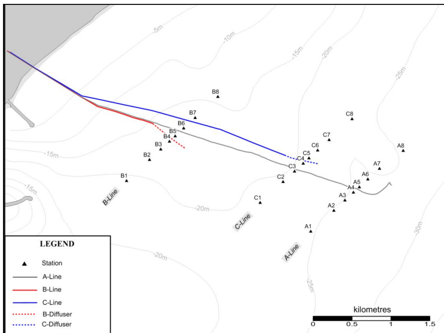
Figure 1. uMngeni-uThukela Water offshore wastewater disposal systems.
